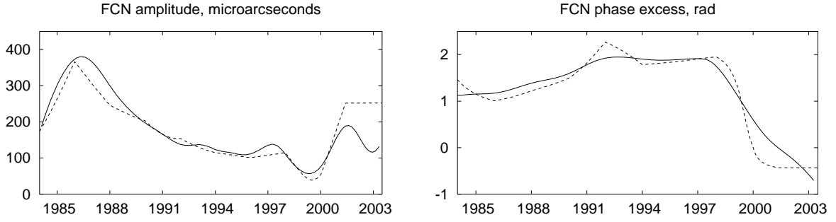
Figure 4: The FCN amplitude and phase (after removing linear trend corresponding to the constant FCN period 430.2^d ) variations found in this study (solid line), and the MHB2000 model (dashed line).
