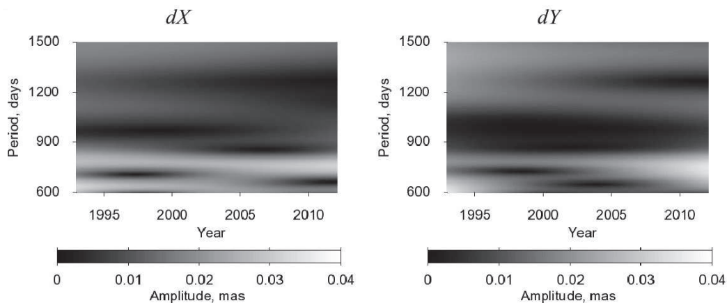
Figure 2: Wavelet scalograms for the IVS combined CPO series after removing FCN.
