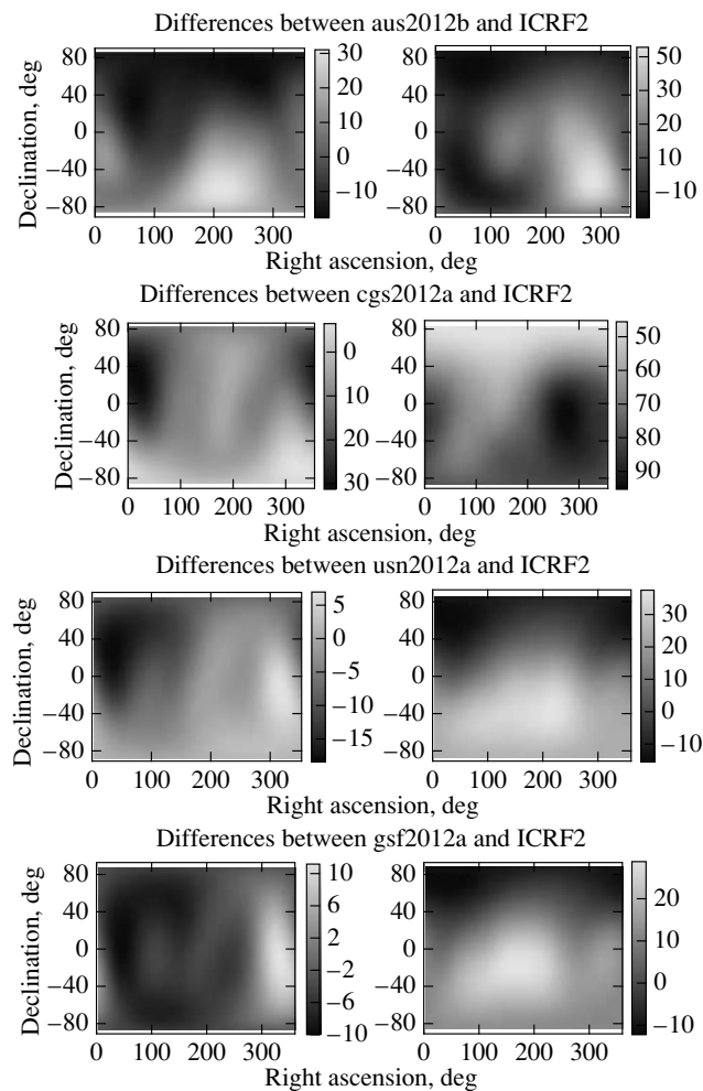
Fig. 4. Smoothed differences between the individual catalogues and ICRF2 in \mu\text{as} from 274 reference sources ( \Delta\alpha \cos \delta on the left, \Delta\delta on the right).
